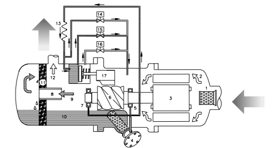
4-step capacity control
