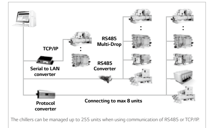
Detailed diagrams of BMS
